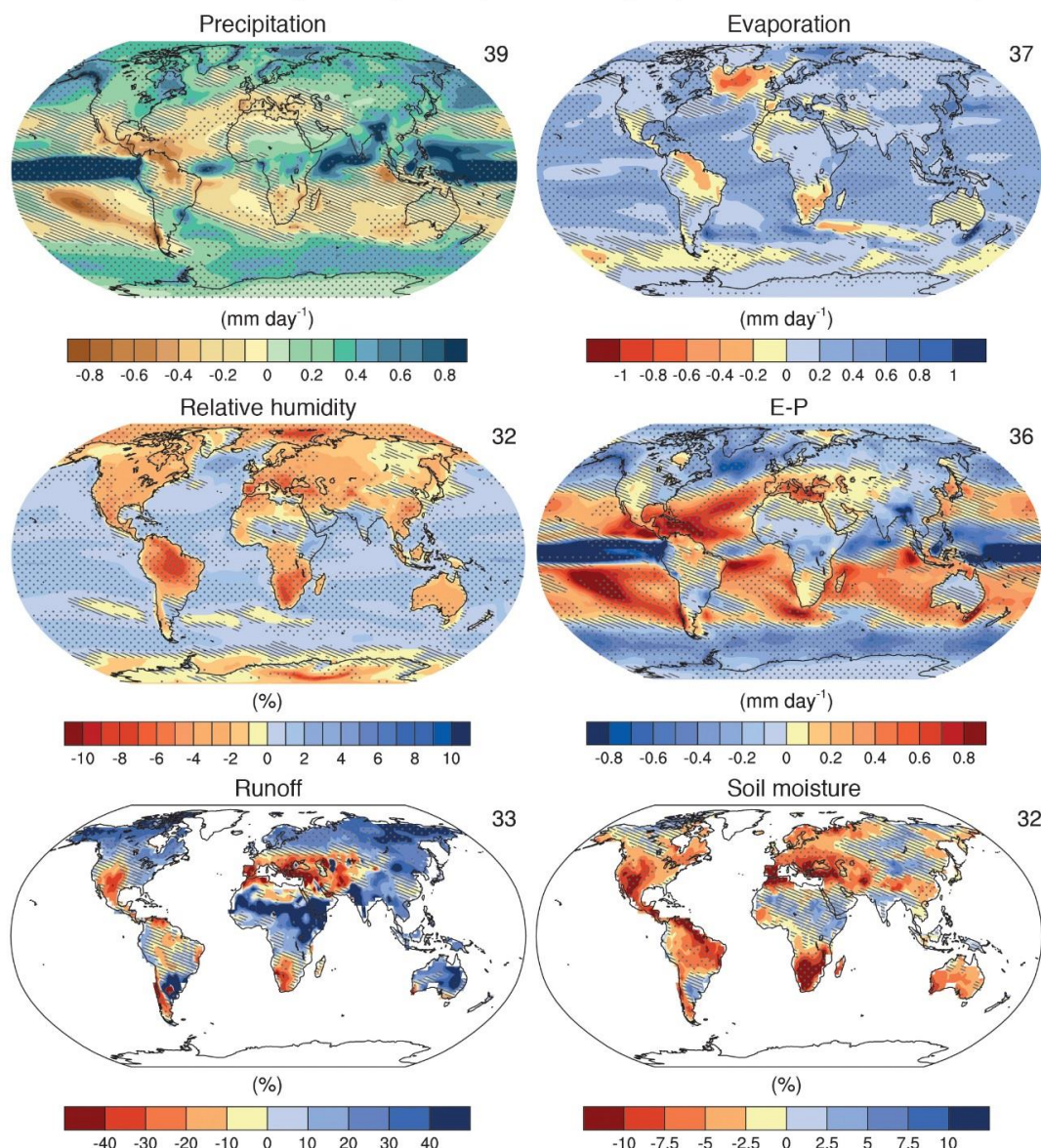
Figure 8: from IPCC, WGI, 2013 Annual mean changes in precipitation (P), evaporation (E), relative humidity, E – P, runoff and soil moisture for 2081–2100 relative to 1986–2005 under the Representative Concentration Pathway RCP8.5. The number of Coupled Model Intercomparison Project Phase 5 (CMIP5) models to calculate the multi-model mean is indicated in the upper right corner of each panel. Hatching indicates regions where the multi-model mean change is less than one standard deviation of internal variability. Stippling indicates regions where the multi-model mean change is greater than two standard deviations of internal variability and where 90% of models agree on the sign of change.
